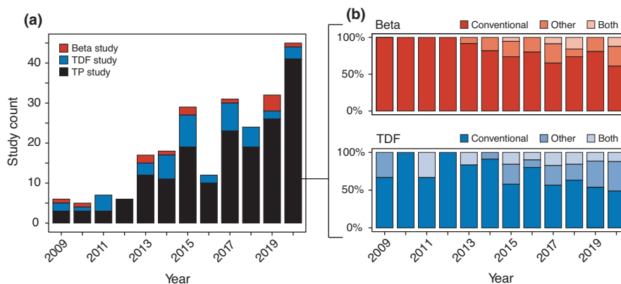
FIGURE 2 (a) Frequency distribution showing the growing number of published studies that use compound-specific stable isotope analysis of amino acids (CSIA-AA) to estimate consumer trophic position ( \text{TP}_{\text{CSIA}} ; black bars, Equation 1, n = 176 ) and parameters of the \text{TP}_{\text{CSIA}} equation [Trophic discrimination factor (TDF), blue bars, n = 44 ; \beta , red bars, n = 15 ]. (b) Percent stacked bar charts illustrating the frequent use of conventional TDF and \beta values in \text{TP}_{\text{CSIA}} calculations, including the lagged consideration of non-conventional \beta values relative to non-conventional TDFs. Conventional indicates use of values from Chikaraishi et al. (2009, 2010; e.g. TDF = 7.6\text{‰} , \beta = +3.4 or -8.4\text{‰} ); Other indicates use of non-conventional parameter values from other studies [e.g. Nielsen et al. (2015), Bradley et al. (2015), study-specific analysis, \beta_{\text{mix}} ]; or Both (e.g. study uses a multi-TDF or multiple equations to calculate \text{TP}_{\text{CSIA}} )
