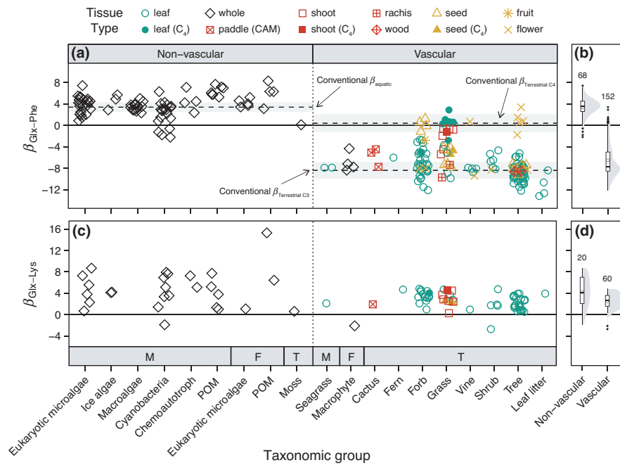
FIGURE 3 (a, c) \beta_{\text{Glx-Phe}} and \beta_{\text{Glx-Lys}} values collated from the published literature illustrating key sources of variability examined in this meta-analysis, including the presence/absence of a vascular system (subpanels), taxonomic group (jittered symbols), habitat type (M = marine, F = freshwater, T = terrestrial), tissue type (T only; colours, symbols) and mode of photosynthesis (T only; all \text{C}_3 unless otherwise noted). Dashed lines and shaded ribbons denote the conventionally applied \beta values (mean \pm SD) for aquatic ( 3.4 \pm 0.9\% ; Chikaraishi et al., 2009), terrestrial \text{C}_3 ( -8.4 \pm 1.6\% ; Chikaraishi et al., 2010), terrestrial \text{C}_4 ( 0.4 \pm 1.7\% ; Chikaraishi et al., 2010) primary producers. Particulate organic matter (POM) data are presented for comparison but were excluded from all analyses. (b, d) Half violin plots with inset boxplots showing the distribution of \beta values for vascular and non-vascular primary producers. Open circles denote groups means. Sample sizes are presented above each plot
